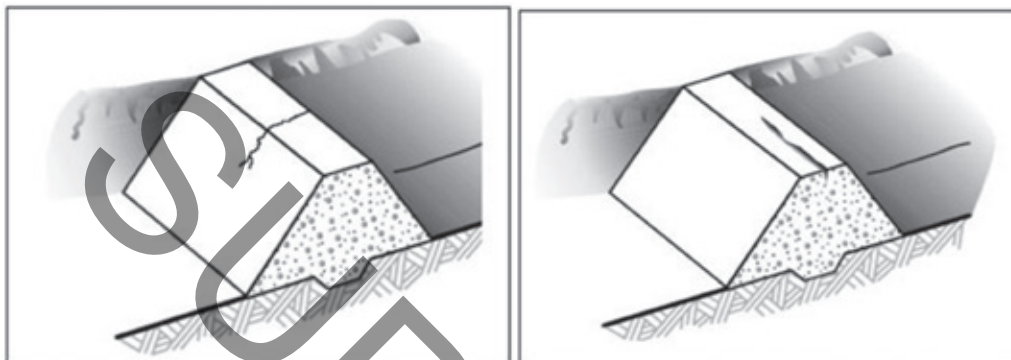
Figure 6.1: Longitudinal and Transverse Cracking (from USFWS 2008).
