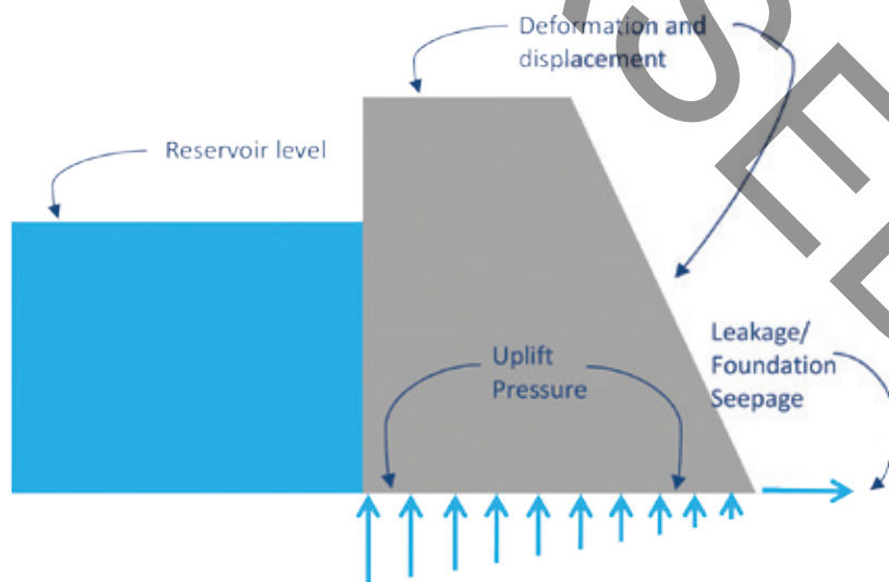
Figure 4.3: Concrete Dam Performance Parameters
